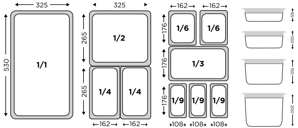
BO 171 High Heat Pans
